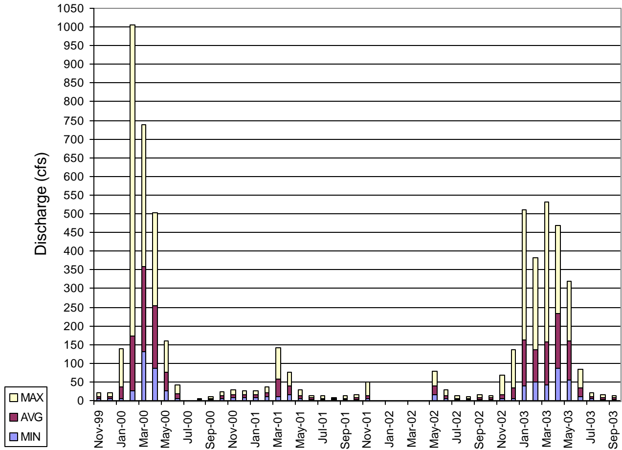
Red Clover Cr@Notson Br; Monthly Summaries of Avg Daily Flow
