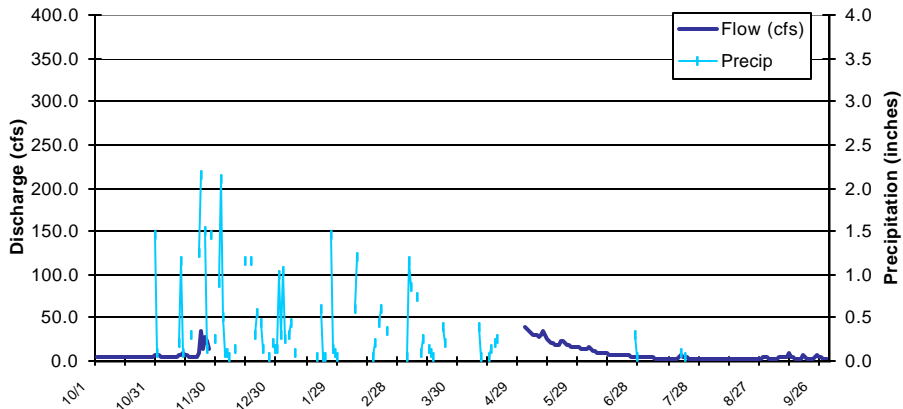
Red Clover Creek at Notson Bridge Daily Average Flow and precipitation at Genesee - Water Year 2002
