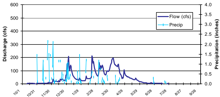
Lights Creek at Deadfall Bridge Daily Average Flow and Precipitation at Genesee - Water Year 2002
